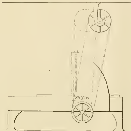
IMPROVING A PLANER.
